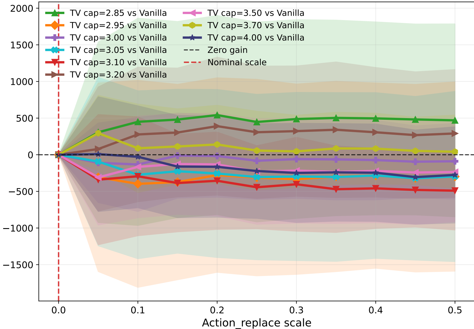
Action_replace robust gain
